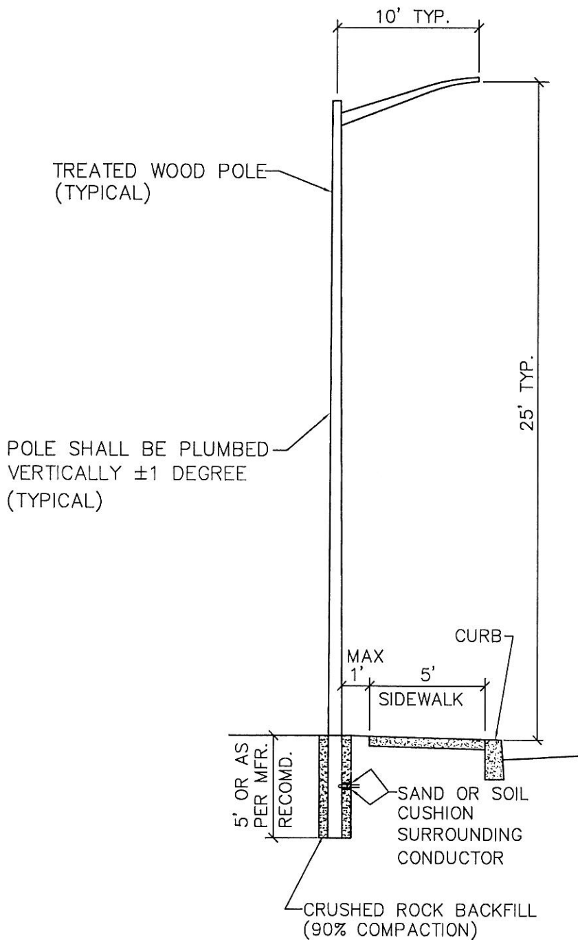
TYPICAL LAMP POST CROSS SECTION TYPE ONE
